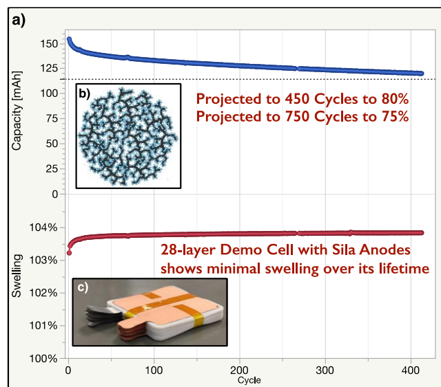
Figure 1. (a) Sila anodes demonstrate excellent cycle life in matched full cells and <1%, cell level swelling over 400+ cycles (b) Sila's technology is based on work published by in 2010 in Nature Materials (c) Sila's stacked demo cell platform uses all commercial components and build methods paired with Sila's proprietary anodes
